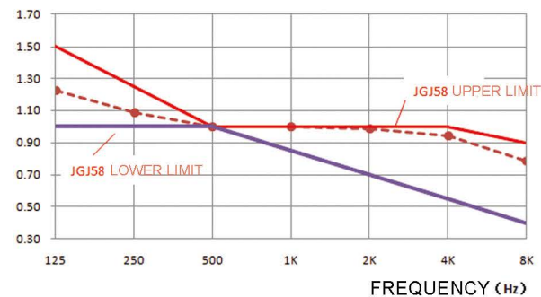
RT60 FREQUENCY SPECTRUM OF NATIONAL STANDARD
