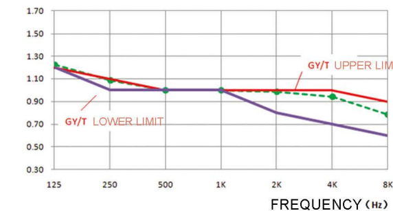
RT60 FREQUENCY SPECTRUM OF INDUSTRY STANDARD
