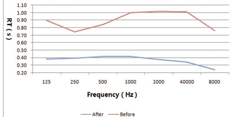
Comparison of RT Curve before and after modification
